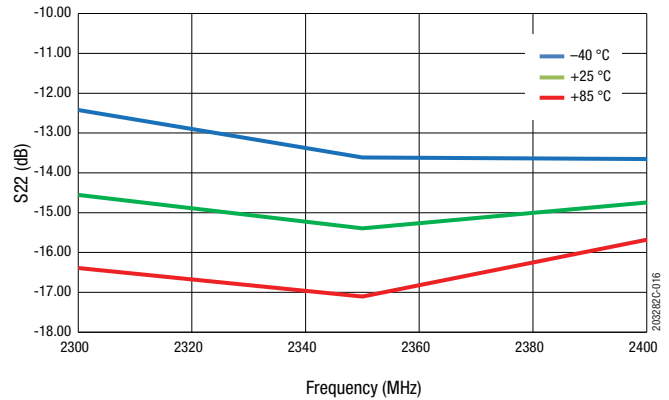
Figure 16. Output Return Loss vs Frequency Across Temperature (Small Signal, P 1M = -20 dBm)
