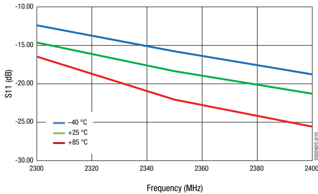
Figure 15. Input Return Loss vs Frequency Across Temperature (Small Signal, P 1M = -20 dBm)
